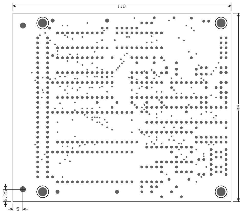
Mechanical Layer 1
