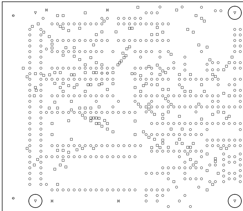
Drill Drawing
